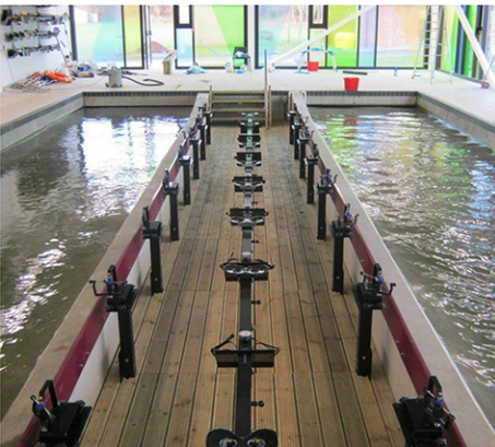
Durham Univ. Boat Club (UK) rowing tank, built by Dreher Boat Company, NH, 2011
